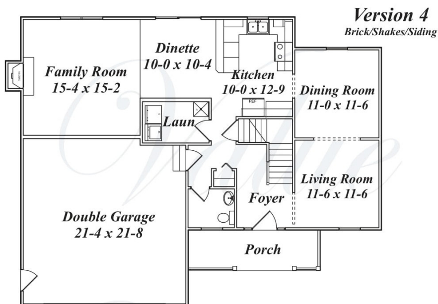
Base First Floor Plan 1025 Square Feet
